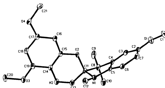
Fig. 5. Crystal structure of (2). The atoms are drawn with 30% probability ellipsoids.
